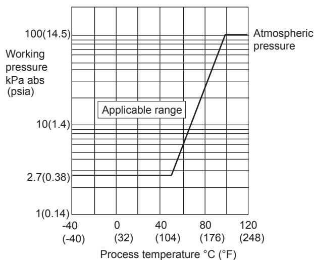
Figure 1-2. Working Pressure and Process Temperature [For EJA530E]
